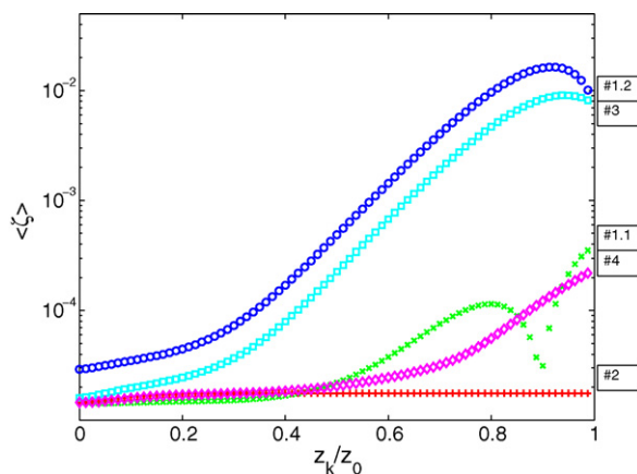
Fig. 6. Averaged anharmonic contribution \langle \zeta(z_k) \rangle along the trap axis for the configurations #1.1, #1.2, #2. Configurations #3 and #4 are introduced later in the text. Strong differences between the trap configurations appear from z_k/z_0 > 0.2 . For clarity, only every 4 th node is plotted.
